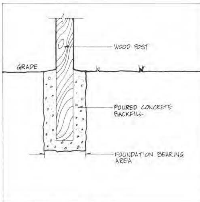
Figure 4.10. Concrete Backfill
