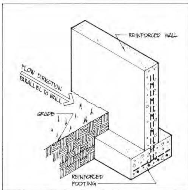
Figure 4.18. Wall Foundation
