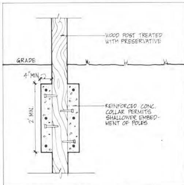
Figure 4.5. Reinforced Concrete Collar
