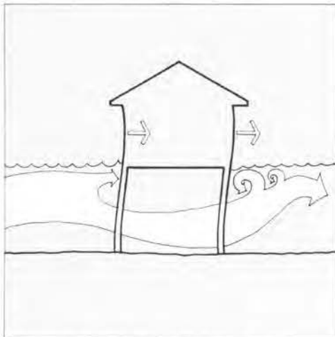
Figure 2.2. Hydrodynamic Forces
