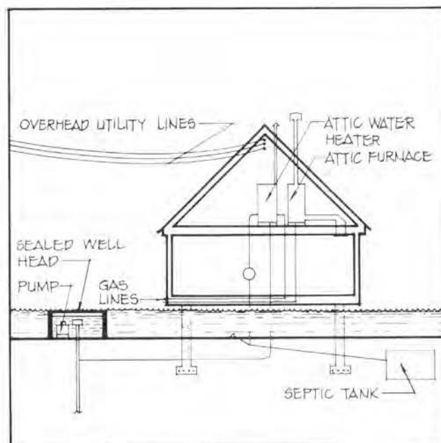
Figure 4.50. Locating Utilities
