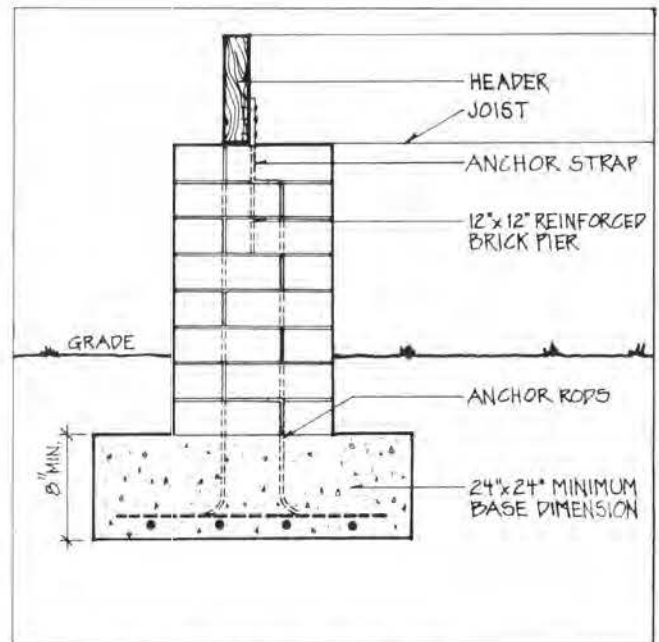
Figure 4.16. Reinforced Brick Pier
