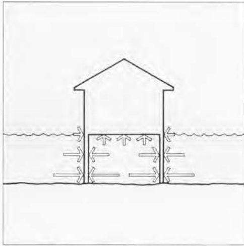
Figure 2.1. Hydrostatic Forces
