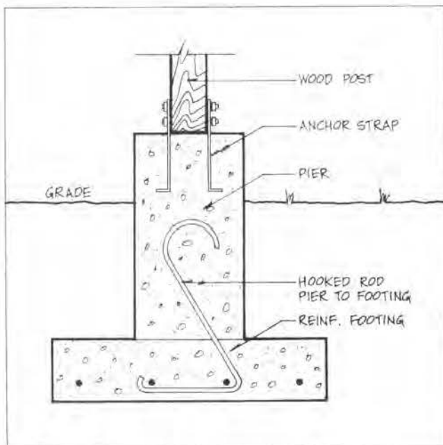
Figure 4.9. Post/Pier Foundation
