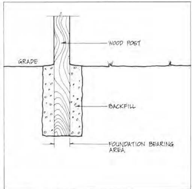
Figure 4.6. Earth Bearing
