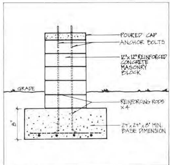
Figure 4.17. Reinforced Concrete Masonry Pier
