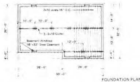
Figure 5.1. Conventional Foundations (Estimates are spring 1983.)
